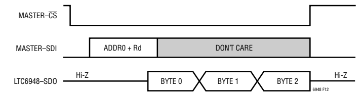
Figure 12. Serial Port Auto-Increment Read
