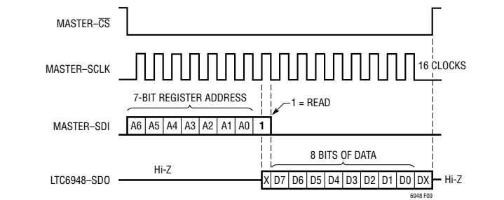
Figure 9. Serial Port Read Sequence
