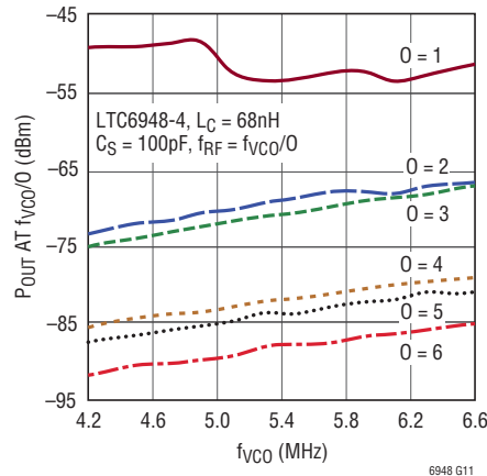
MUTE Output Power vs f_{\text{VCO}} and Output Divide (Single-Ended on RF + )
