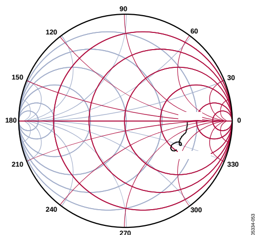
Figure 37. Differential Input Impedance (S11) vs. Frequency; Z_0 = 50\Omega
