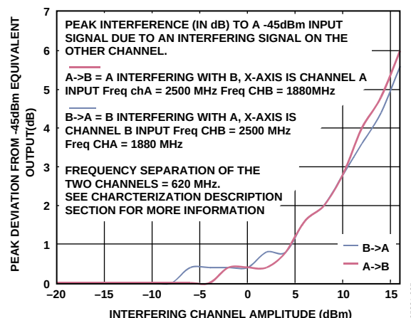
Figure 75. Improved Measurement Error with Increased Frequency Separation
