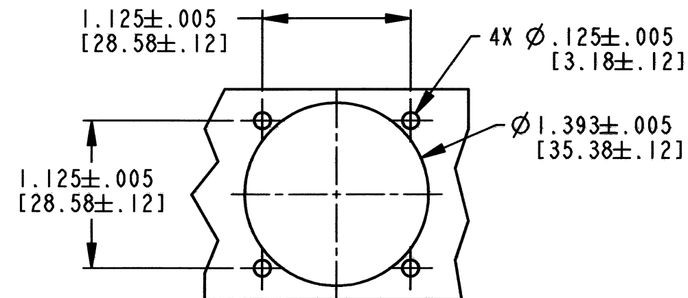
RECOMMENDED PANEL CUTOUT 4
