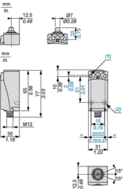
(1) 2 elongated holes Ø 4.3 x 6.3 mm on 22 mm centres, 2 holes Ø 4.3 on 20 mm centres.
