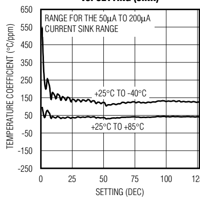
TEMPERATURE COEFFICIENT vs. SETTING (SINK)
