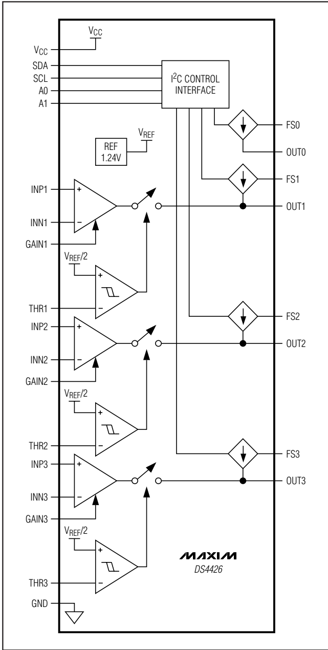
Functional Diagram
