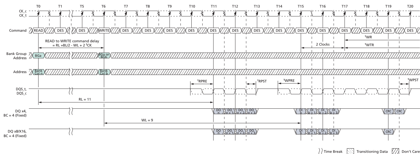
Figure 161: READ (BC4: Fixed) to WRITE (BC4: Fixed) with 1 st CK Preamble and Write CRC in Same or Different Bank Group
