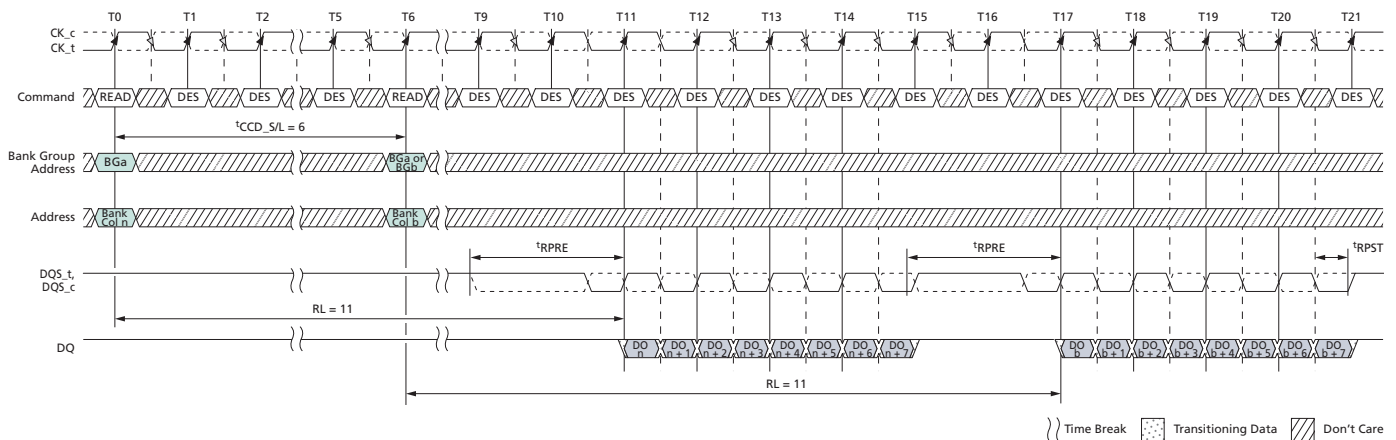
Figure 135: Nonconsecutive READ (BL8) with 2 nd CK Preamble in Same or Different Bank Group
