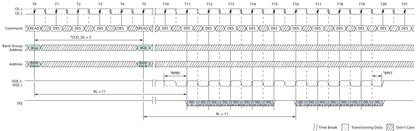
Figure 134: Nonconsecutive READ (BL8) with 1 st CK Preamble in Same or Different Bank Group
