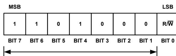
FIGURE 5. I 2 C SLAVE ADDRESS
