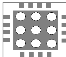
FIGURE 4. EXPOSED THERMAL PAD
