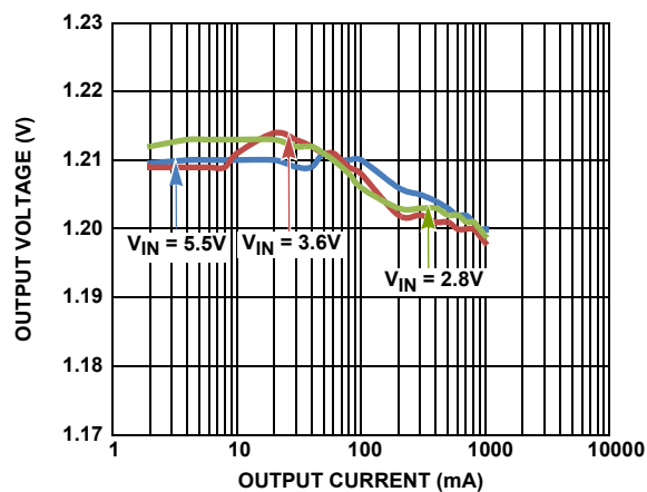
FIGURE 16. DCD OUTPUT VOLTAGE vs LOAD ( V_{OUT} = 1.2V , PFM/PWM)
