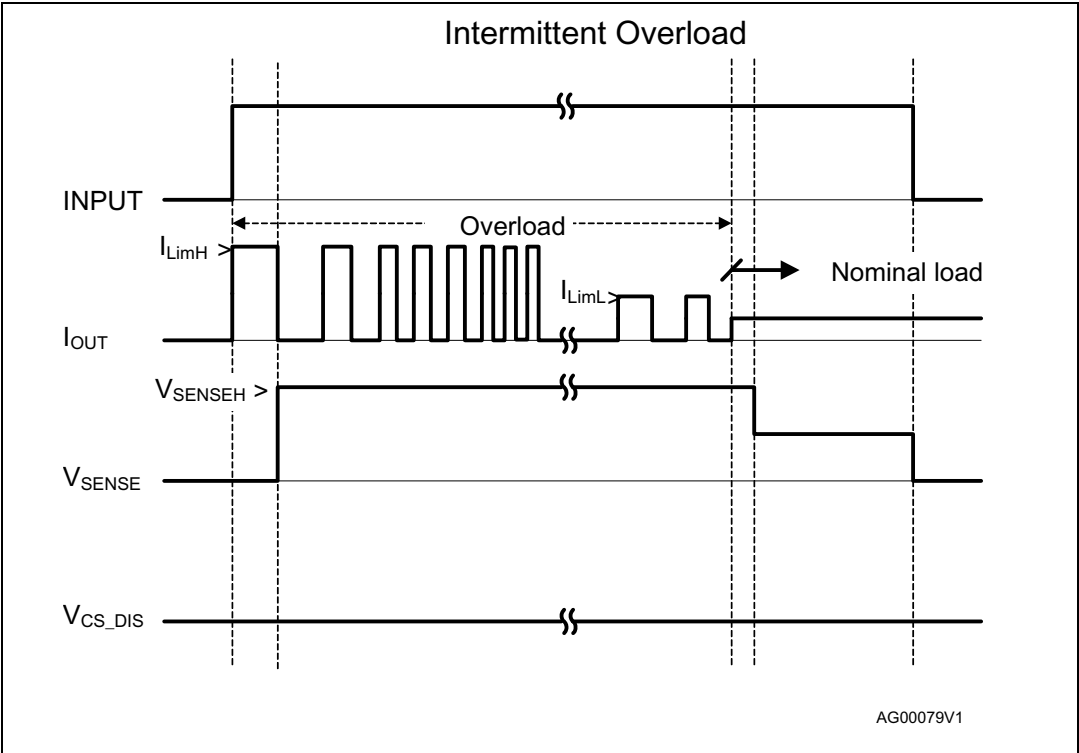
Figure 13. Intermittent overload
