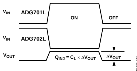
Figure 17. Charge Injection
