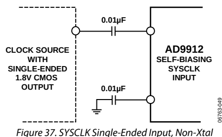
Figure 37. SYSCLK Single-Ended Input, Non-Xtal
