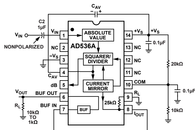
Figure 17. Single-Supply Connection
