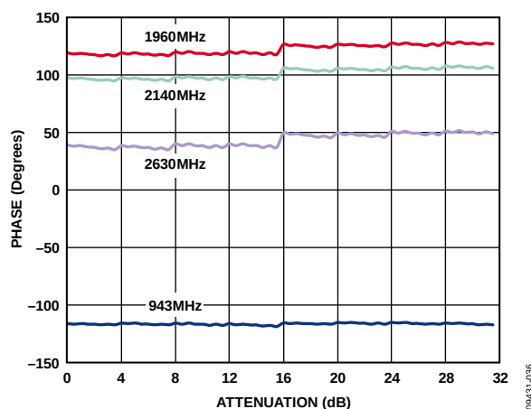
Figure 36. DSA: Phase vs. Attenuation
