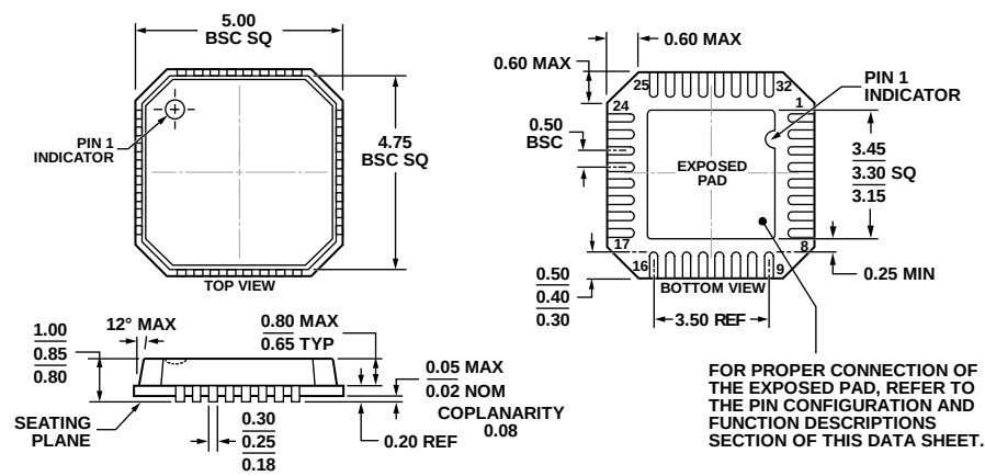
COMPLIANT TO JEDEC STANDARDS MO-220-VHHD-2 Figure 80. 32-Lead Lead Frame Chip Scale Package [LFCSP_VQ] 5 mm x 5 mm Body, Very Thin Quad (CP-32-3) Dimensions shown in millimeters
