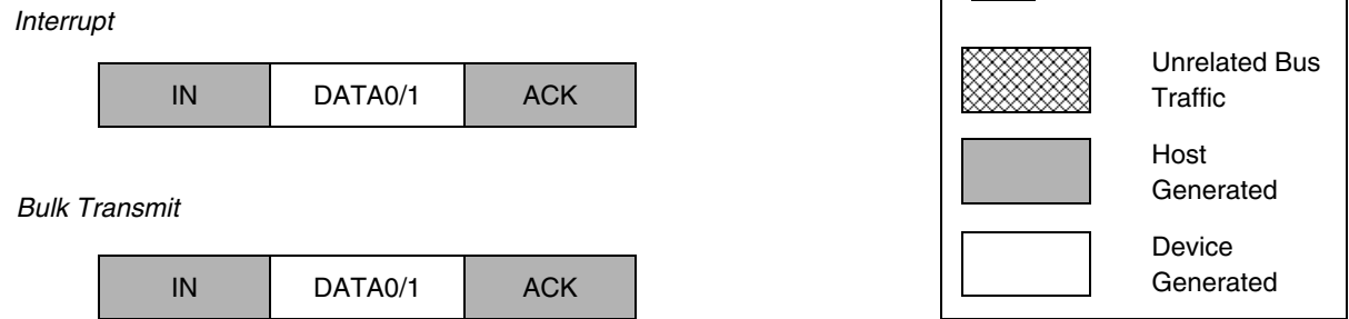
Figure 9-3. Supported Transaction Types Per Endpoint
