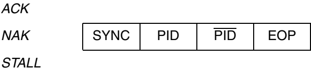
Figure 9-4. Supported USB Packet Types
