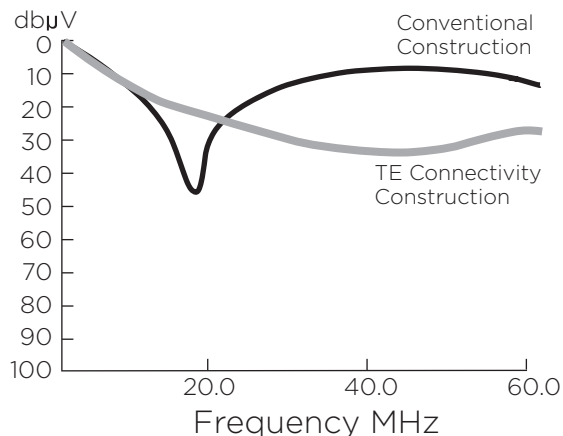
Figure 1: Insertion Loss
