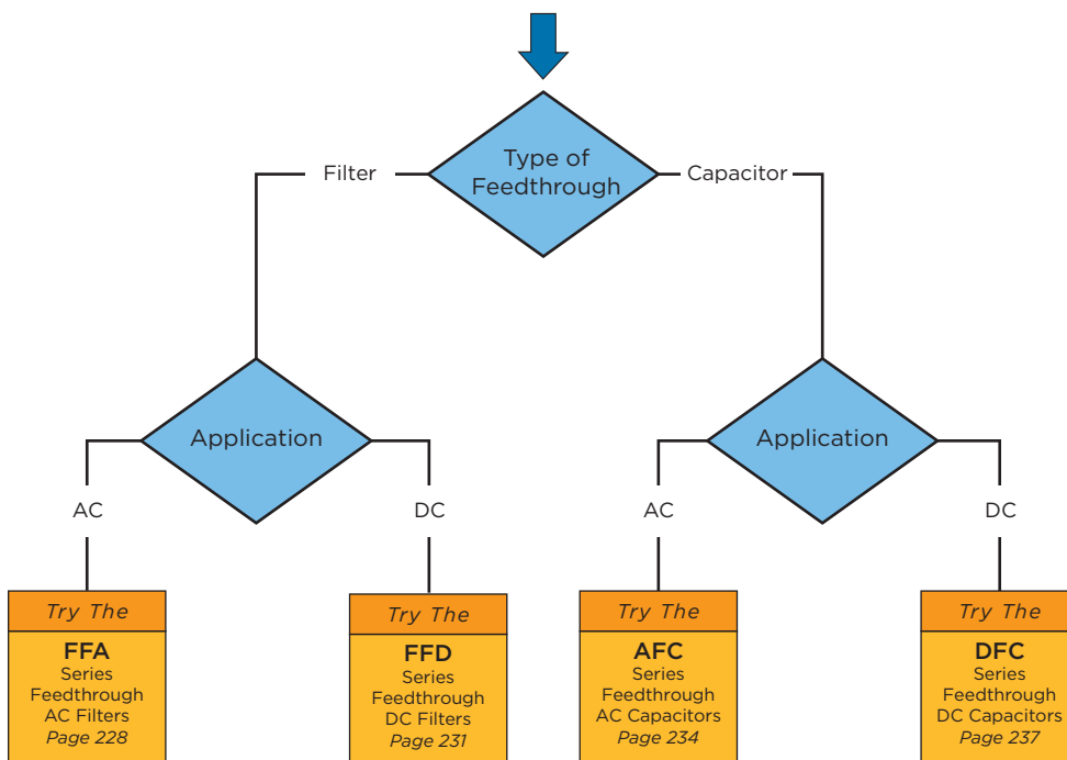
Feedthrough Application Selector Chart
