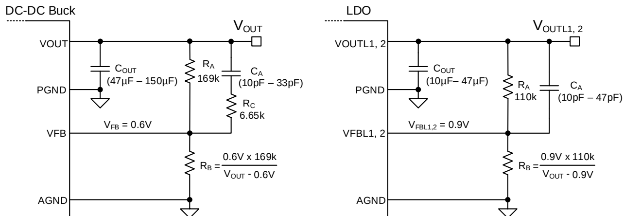
Figure 6: Output Voltage Setting (Buck left, LDO right)
