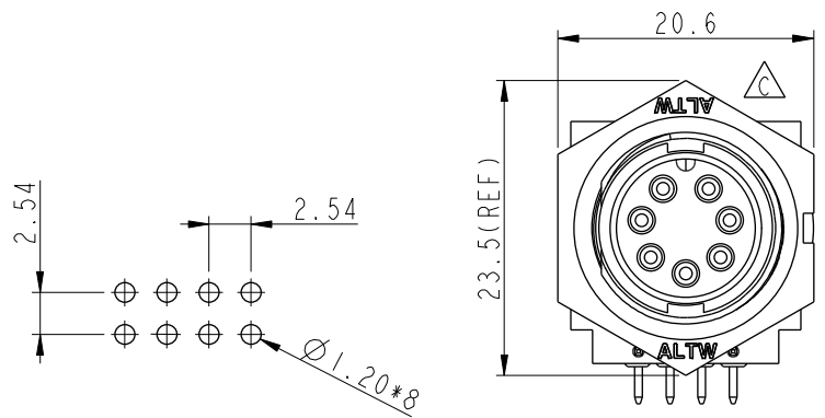
7 Pin Male Connector Male Pin PCB Layout
