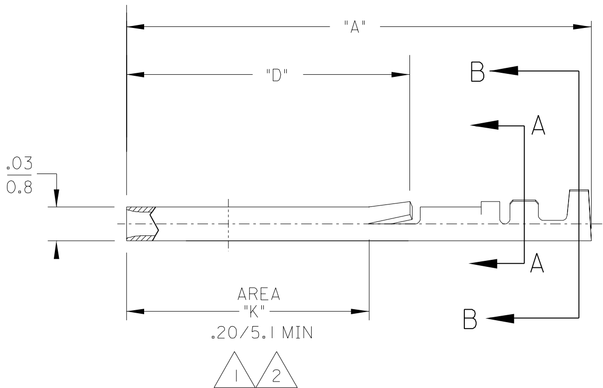
CARRIER DETAIL
