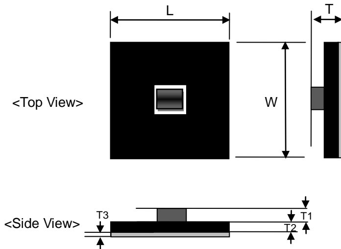
Fig.2 Package Dimension
