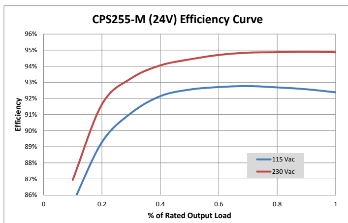
Figure 4. Typical Efficiency for 24 V Output
