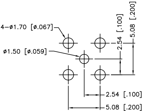
PCB MOUNTING HOLE
