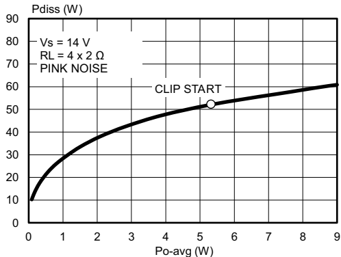
Figure 19. Power dissipation vs. average output power (2 \Omega , audio program simulation)
