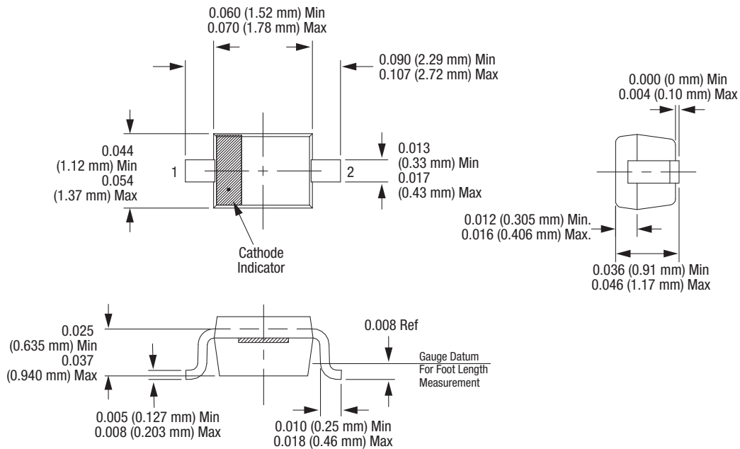
Dimensions are in inches (millimeters shown in parentheses) 200061T-008
