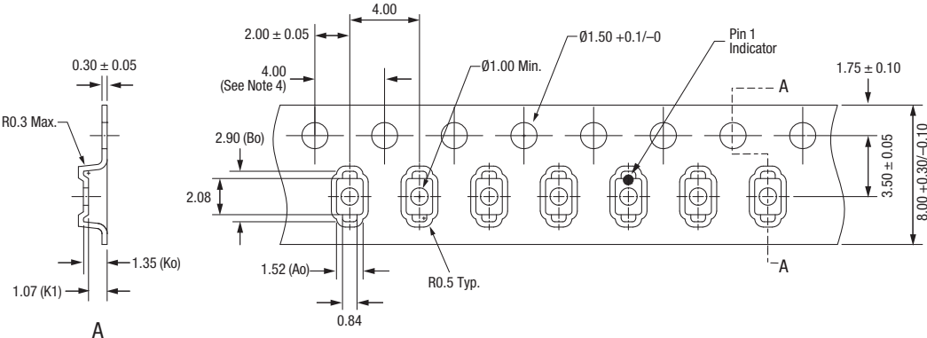
Notes: 1. Carrier tape: black conductive polystyrene. 2. Cover tape: transparent conductive PSA. 3. Cover tape size: 5.4 mm width. 4. 10 sprocket hole pitch cumulative tolerance: ±0.20 mm. 5. All measurements are in millimeters. 200061T-009
