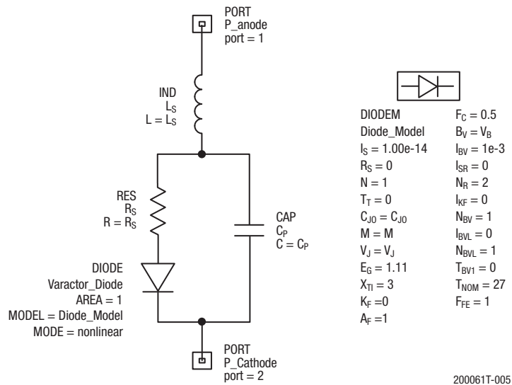
Figure 5. SPICE Model
