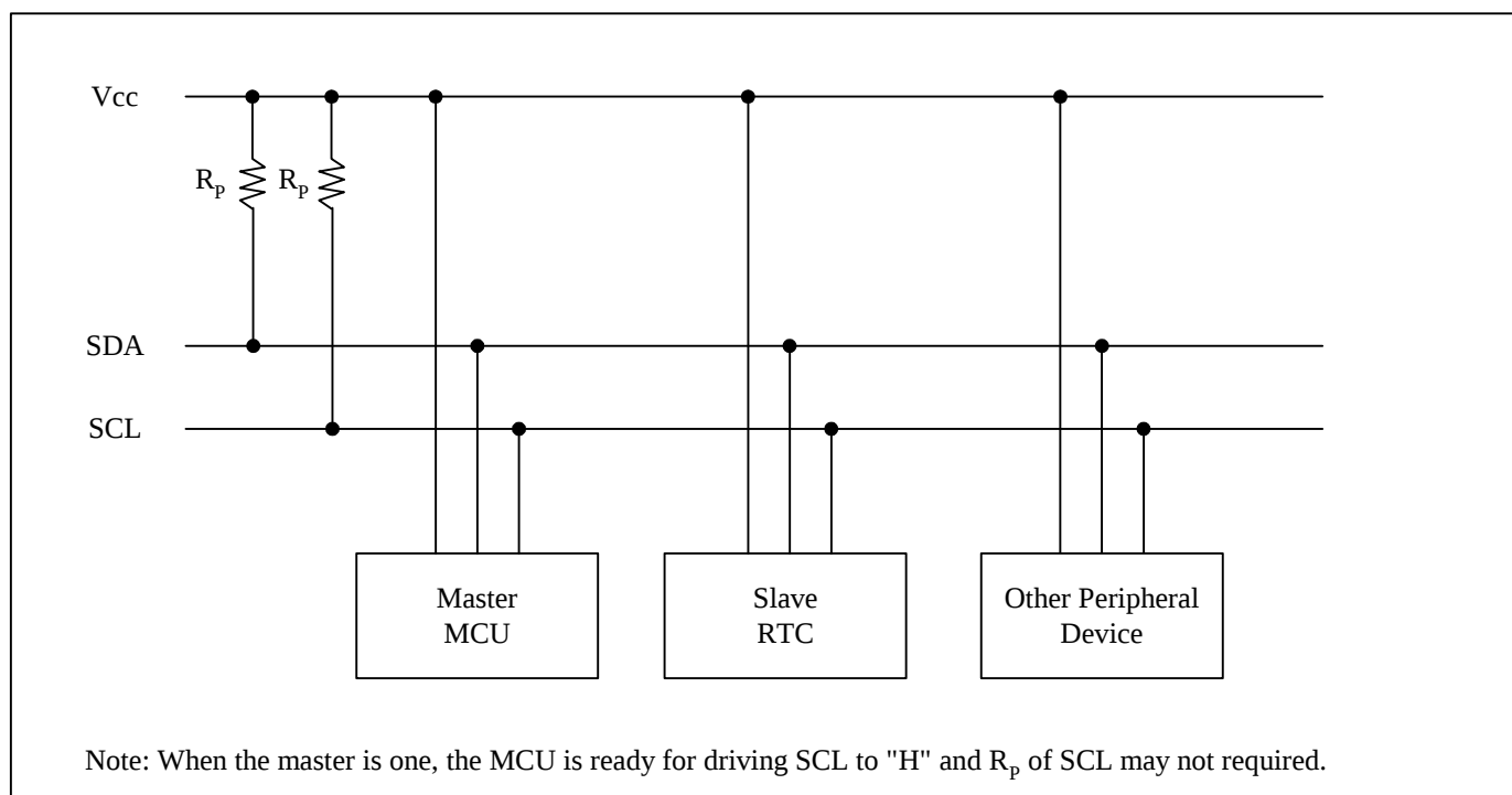
Fig 4. System configuration
