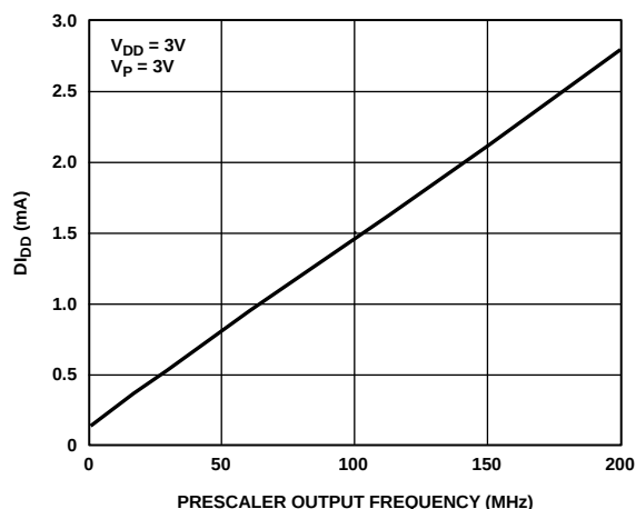
Figure 26. D I_{DD} vs. Prescaler Output Frequency (ADF4110, ADF4111, ADF4112, ADF4113)
