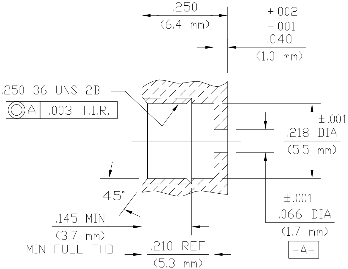
RECOMMENDED MOUNTING HOLE
