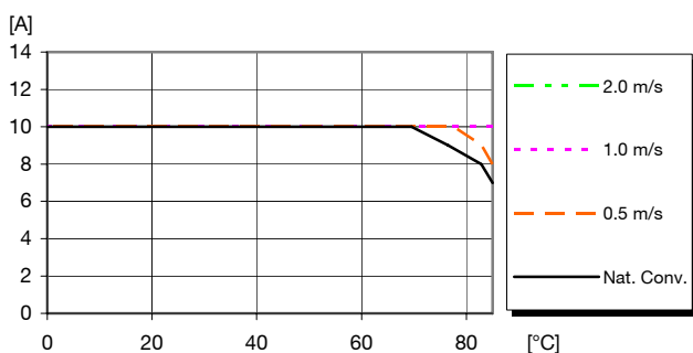
Available load current vs. ambient air temperature and airflow at V_I = 5.0\text{ V} , V_{OUT} = 3.3\text{ V} . See Thermal Consideration section.
