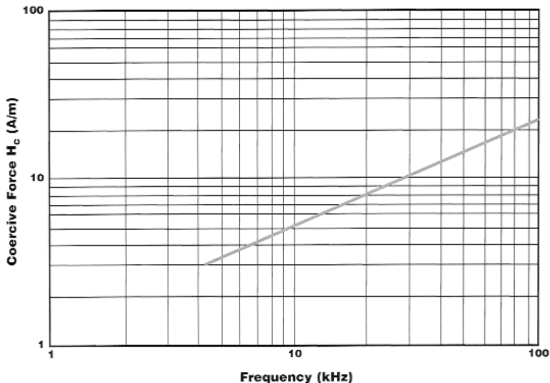
Coercive Force vs. Frequency @ 25°C
