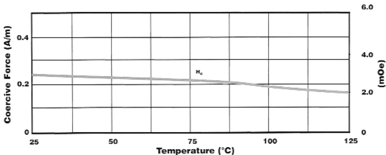
Coercive Force vs. Temperature ††
