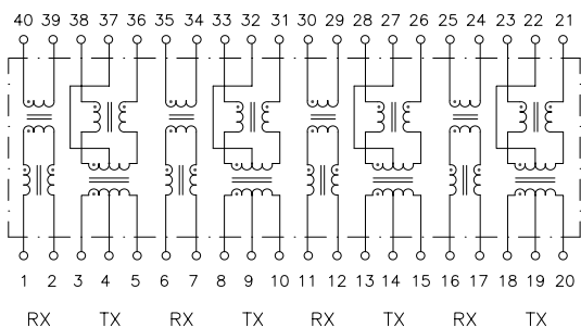
Circuit C
