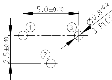
PCB MOUNTING DETAILS
