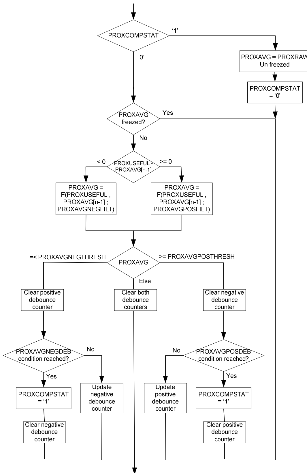
Figure 37 – ProxAvg Update
