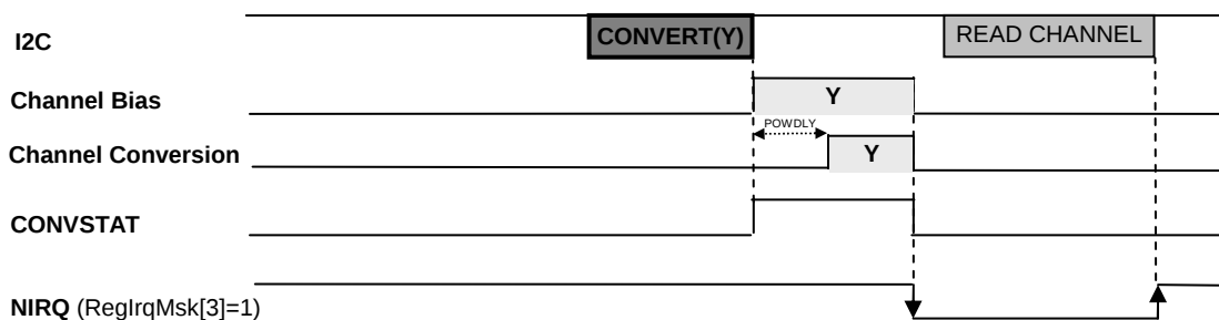
Figure 18 – Manual Mode – CONVERT Command (CHAN = Y; PROXSCANPERIOD = 0)
