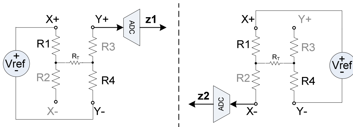
Figure 12 – Pressure Measurement
