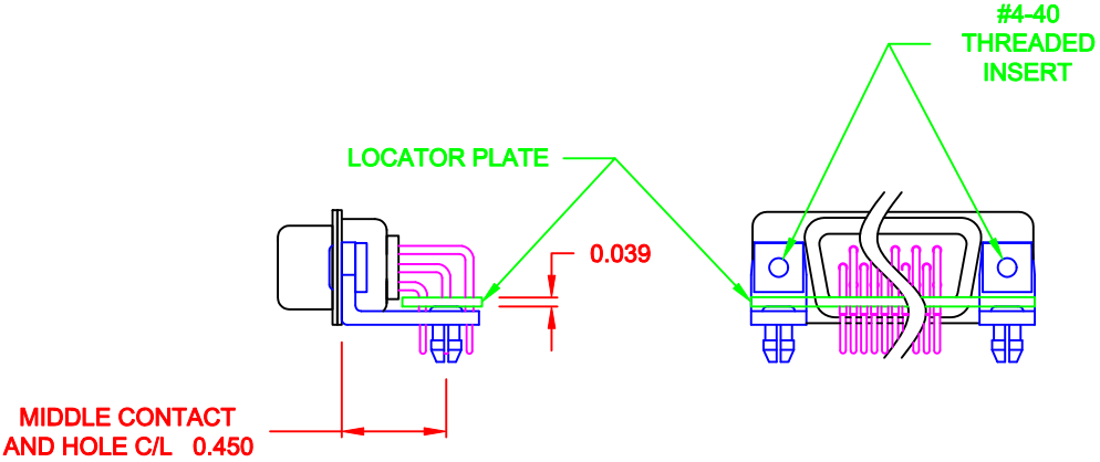
BRACKETS MOUNTED ON CONNECTOR WITH LOCATOR PLATE
