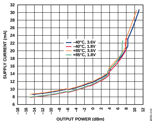
Figure 14. Differential PA at 915 MHz: Supply Current vs. Output Power, Temperature, and V_{DD} (Minimum Recommended V_{DD} = 2.2 V, 1.8 V Operation Shown for Robustness)
