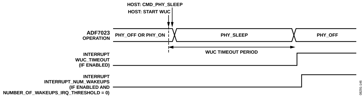
Figure 98. Low Power Mode Timing When Using the WUC
