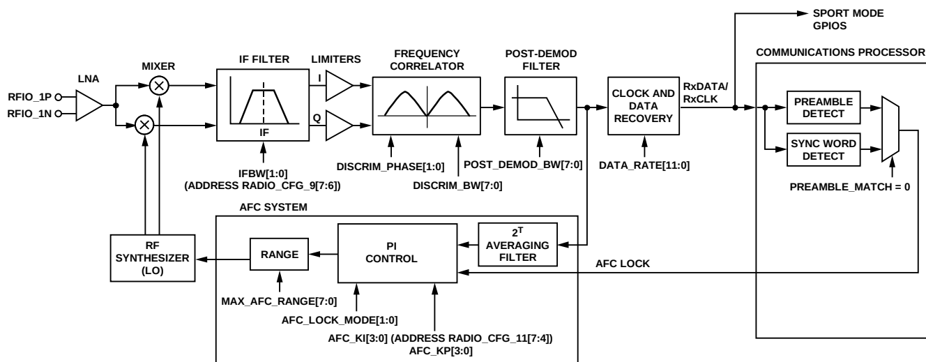
Figure 109. 2FSK/GFSK/MSK/GMSK Demodulation and AFC Architecture
