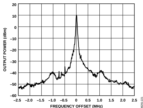
Figure 24. OOK Transmit Spectrum, Max Hold for 100 Sweeps, Single-Ended PA, 868.95 MHz, Data Rate = 16.4 kbps (32.8 kbps, Manchester Encoded), PA_RAMP = 1
