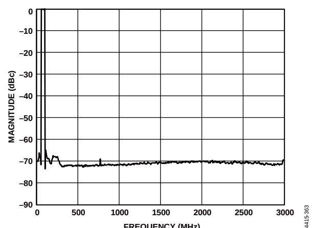
Figure 64. Eight Carriers at 70 MHz Output (Shuffle On)
