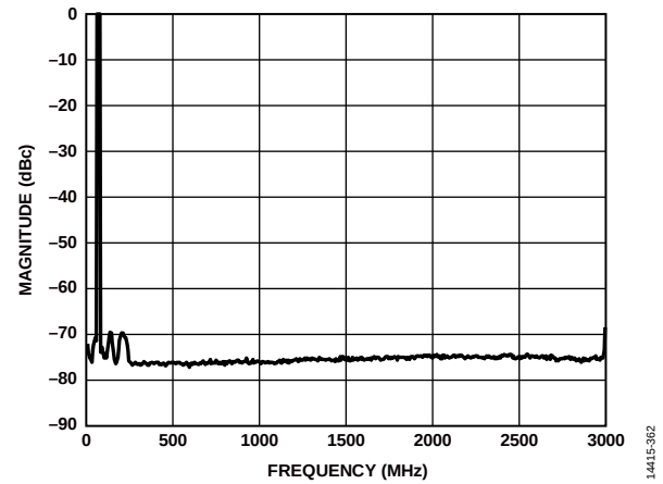
Figure 63. Four Carriers at 70 MHz Output (Shuffle On)
