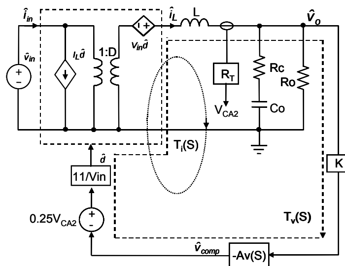
FIGURE 17. SMALL SIGNAL MODEL OF SYNCHRONOUS BUCK REGULATOR
