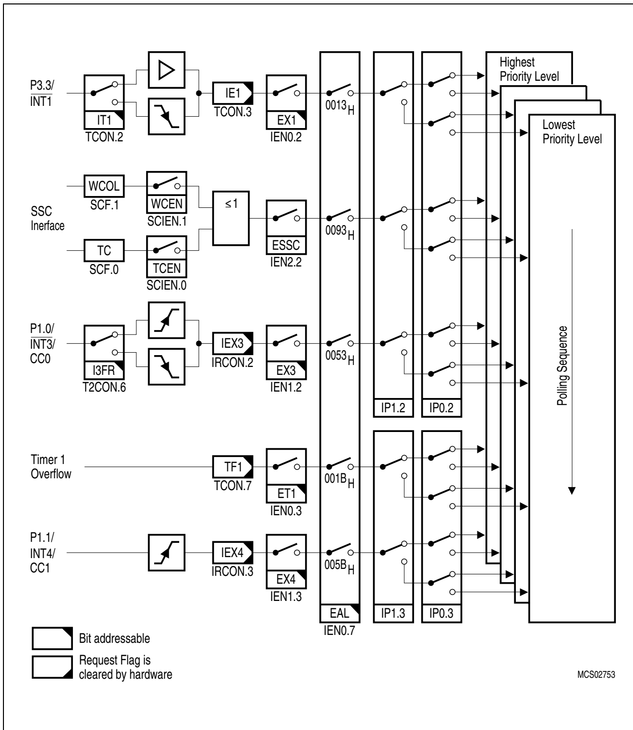
Figure 21 Interrupt Request Sources (Part 2)
