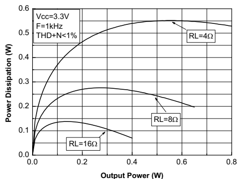
Figure 23. Power dissipation vs P out (V cc = 3.3 V)
