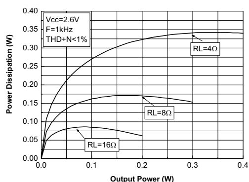
Figure 24. Power dissipation vs P out (V cc = 2.6 V)
