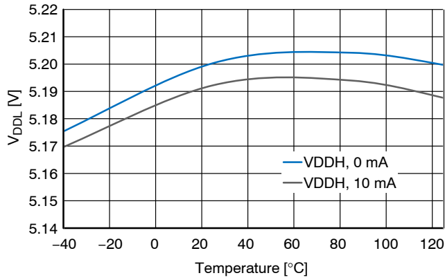
Figure 11. VDDL ( V_{DDL} ) Regulated Output Voltage vs. Temperature
