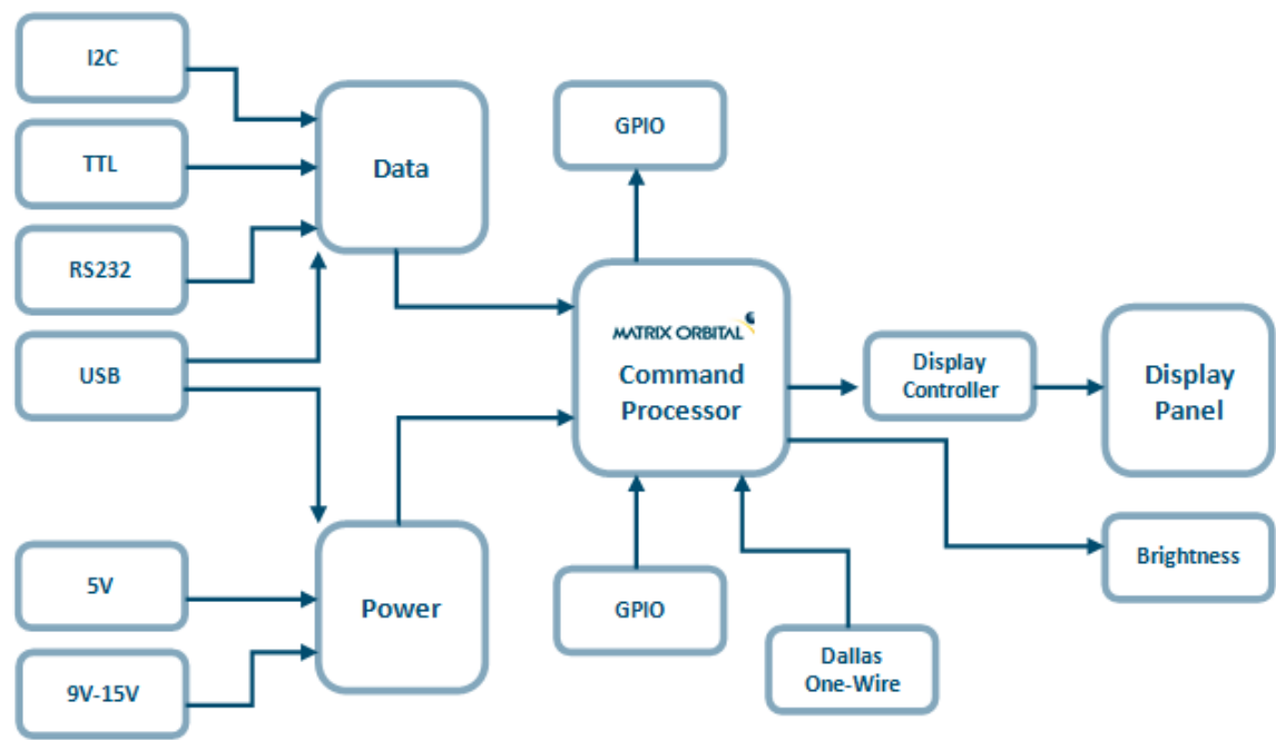
Figure 16: Functional Diagram
