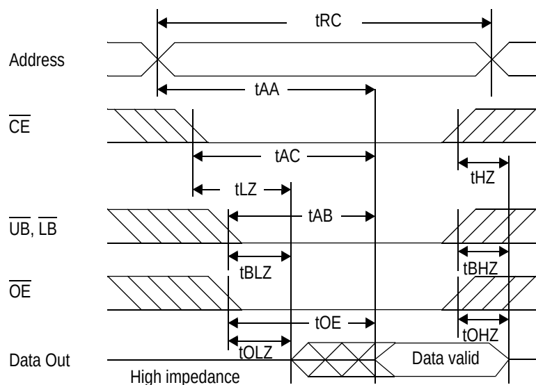
Read Cycle 2: \overline{WE} = V_{IH}
