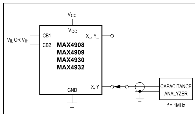
Figure 6. Channel Off/On-Capacitance
