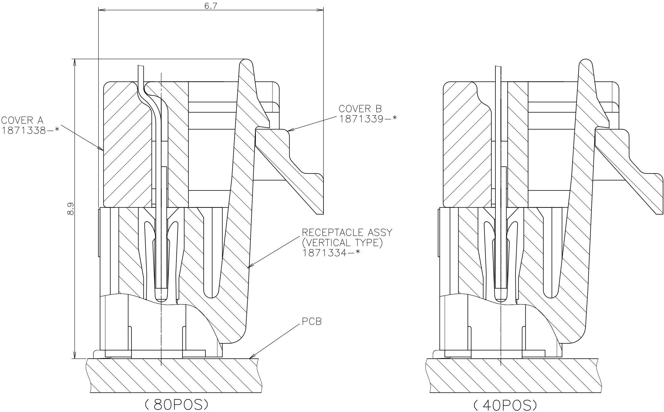
MATING CONDITION
