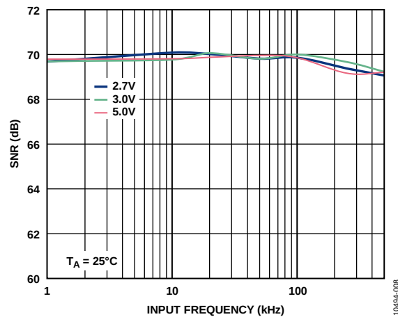
Figure 8. SNR vs. Analog Input Frequency for Various Supply Voltages
