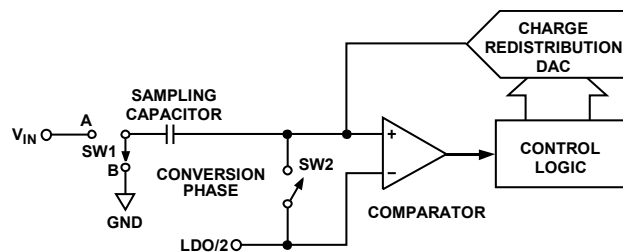
Figure 19. ADC Conversion Phase
