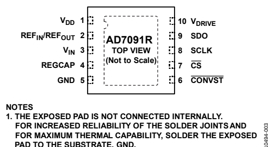
Figure 3. Pin Configuration, 10-Lead LFCSP
