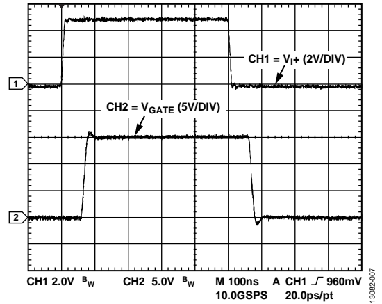
Figure 7. Typical Input to Output Waveform, 2 nF Load, 3.9 \Omega Series Gate Resistor, V_{DD1} = 5V , V_{DD2} = 15V , V_{SS2} = 0V
