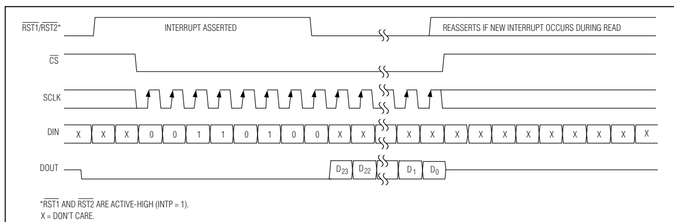
Figure 15. Read of Status Register to Clear Asserted Interrupt ( \overline{\text{RST1}}/\overline{\text{RST2}} )
