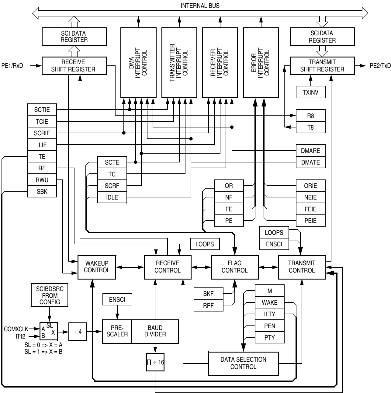
Figure 18-1. SCI Module Block Diagram
