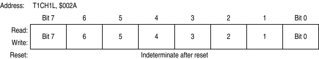
Figure 22-15. TIM Channel 1 Register Low (TCH1L)
