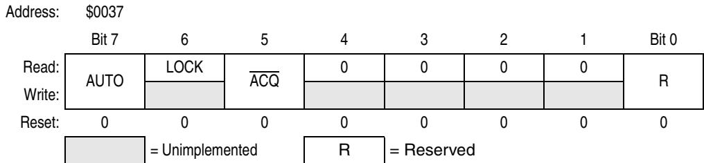
Figure 7-5. PLL Bandwidth Control Register (PBWC)
