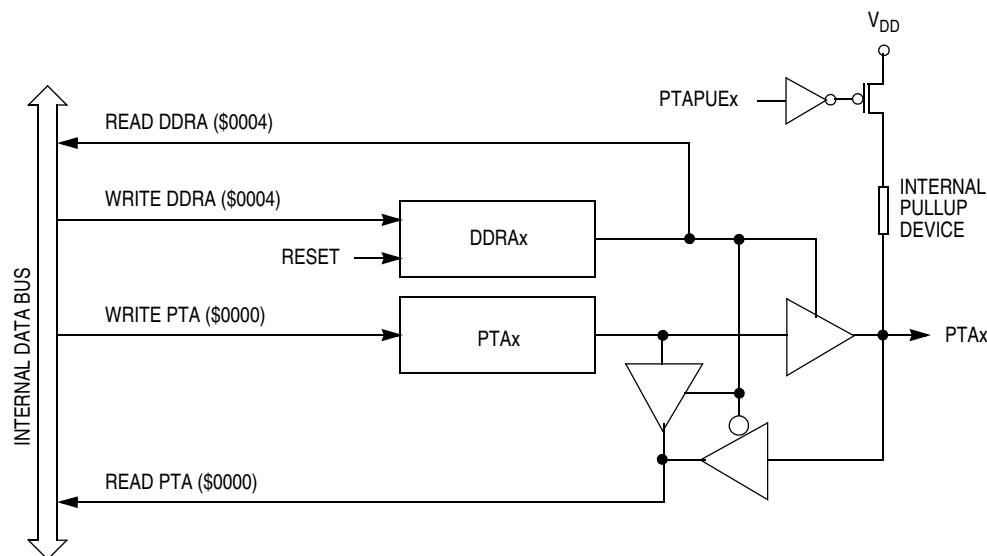
When bit DDRAx is a 1, reading address $0000 reads the PTAx data latch. When bit DDRAx is a 0, reading address $0000 reads the voltage level on the pin. The data latch can always be written, regardless of the state of its data direction bit. Table 16-2 summarizes the operation of the port A pins.
