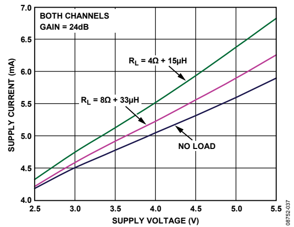
Figure 21. Supply Current vs. Supply Voltage, Gain = 24 dB
